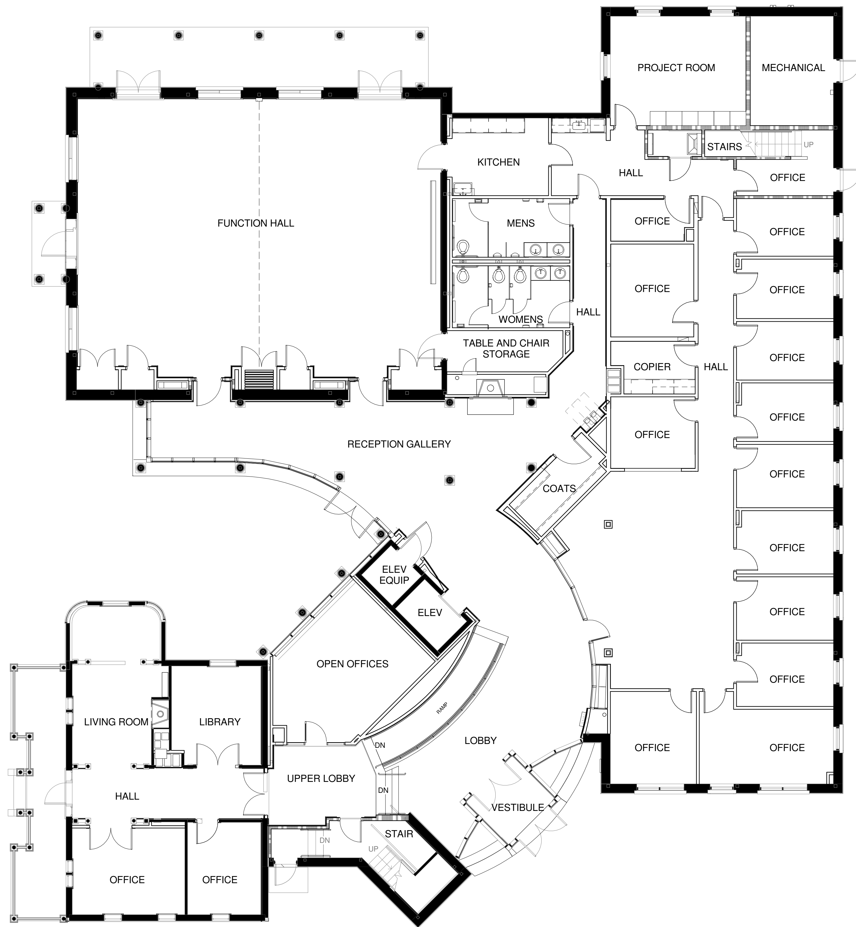
1 First Floor Plan 1/8" = 1'-0"
