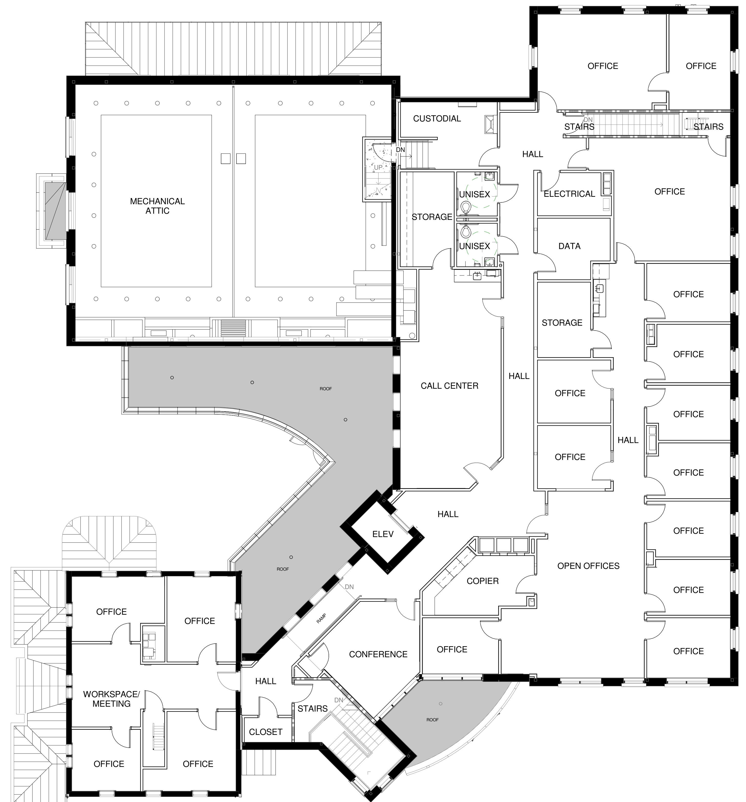
2 Second Floor Plan 1/8" = 1'-0"
